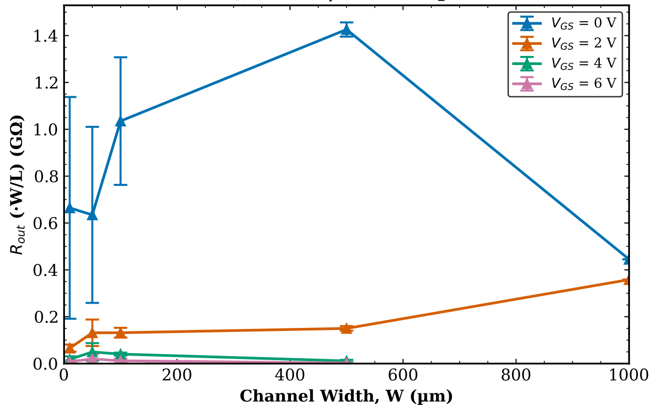
All Chips - Combined R_{out} vs W | L = 160\text{ }\mu\text{m}
